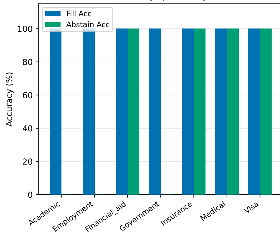
Per-Category Accuracy
